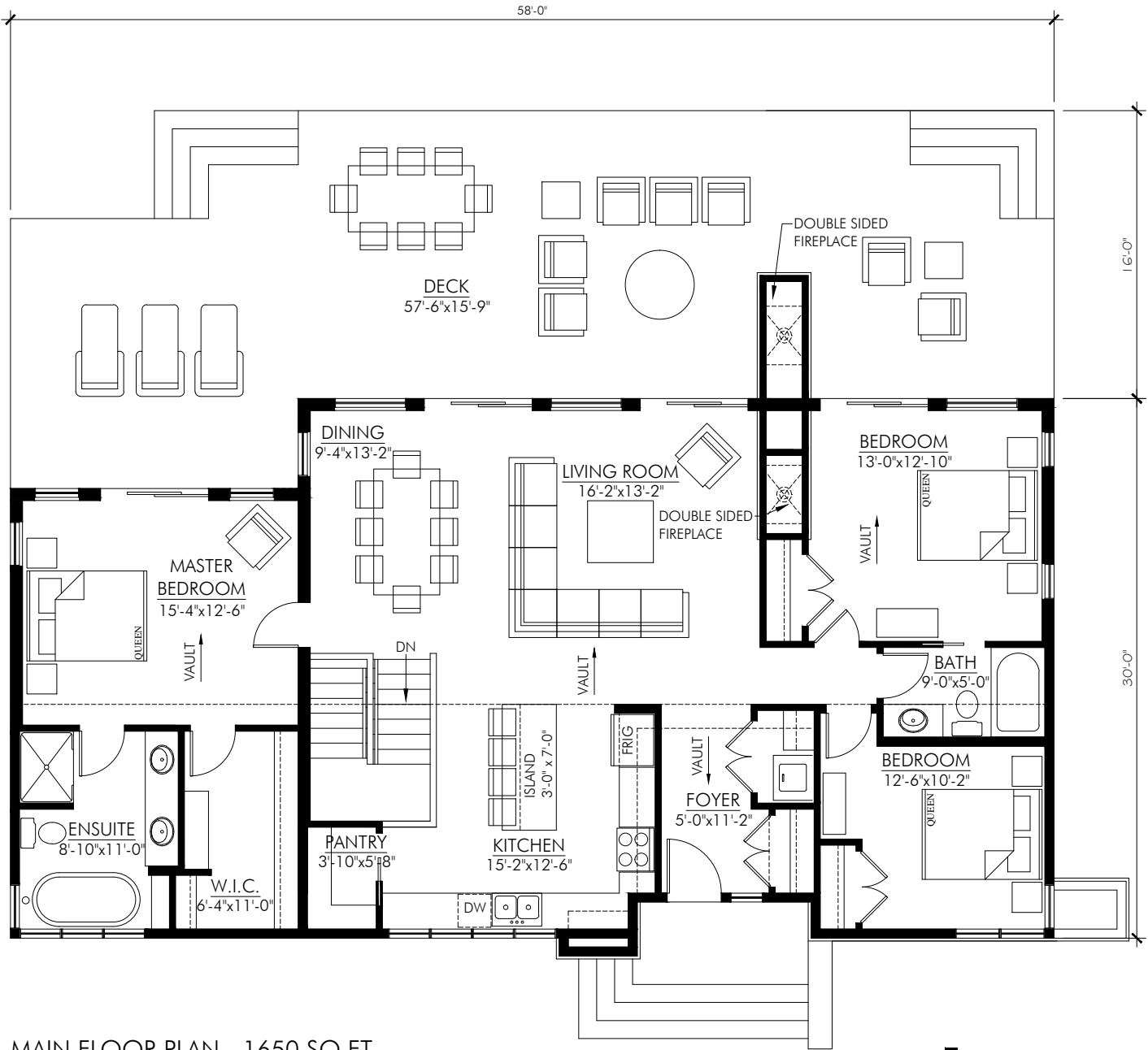
MAIN FLOOR PLAN - 1650 SQ.FT. MONARCH-1650
