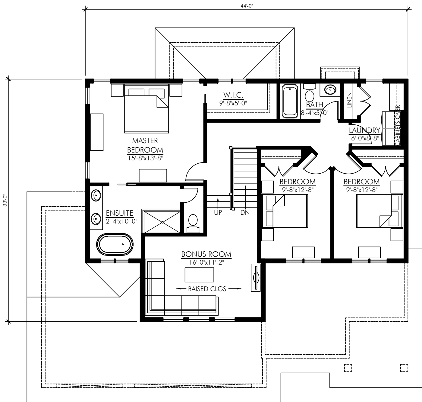
SECOND FLOOR PLAN - 1236 SQ FT SANDFORD-2463
