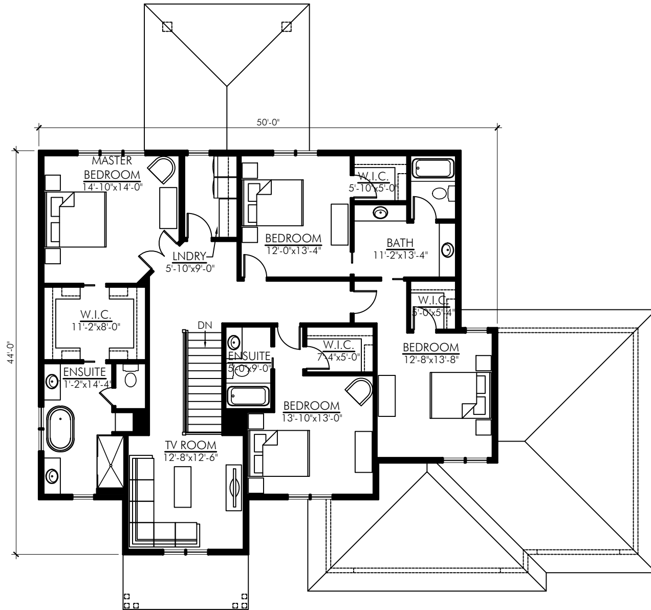
SECOND FLOOR PLAN - 1853 SQ. FT. BRIGHTON-3431
