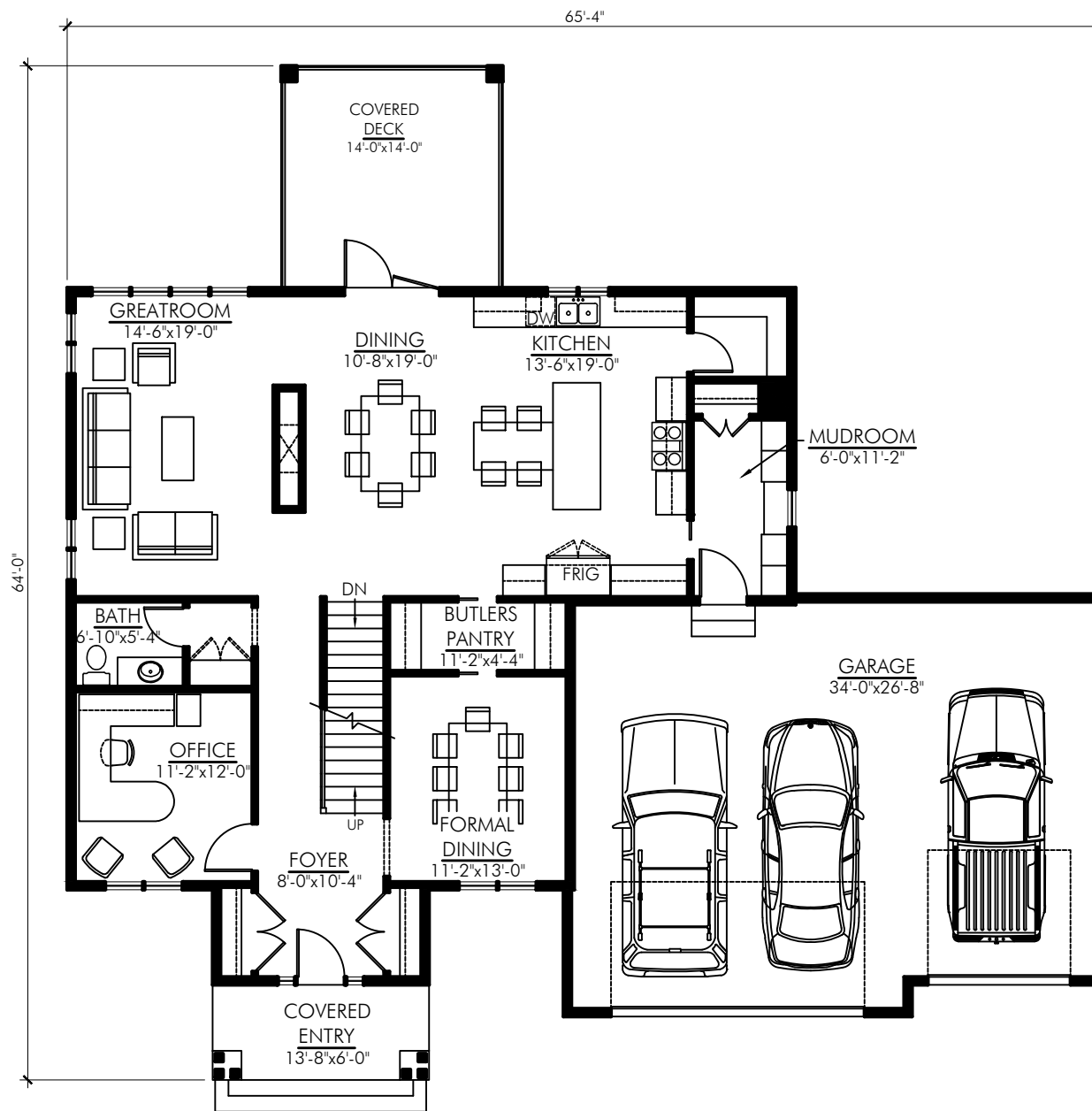
MAIN FLOOR PLAN - 1578 SQ. FT. BRIGHTON-3431
