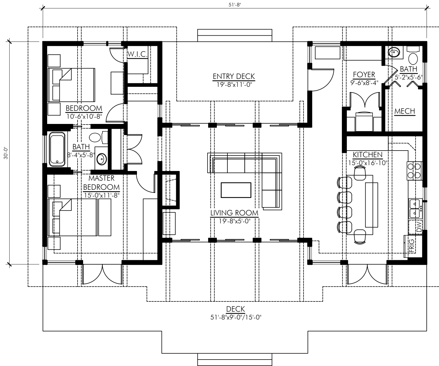
MAIN FLOOR PLAN - 1275 SQ. FT. NOKOMIS-1275
