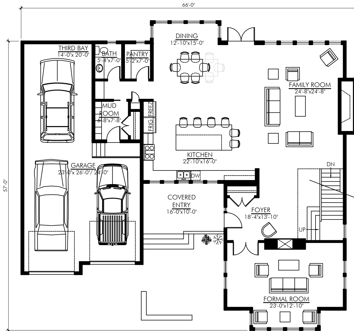
MAIN FLOOR PLAN - 2035 SQ. FT. LOWRY-3512
