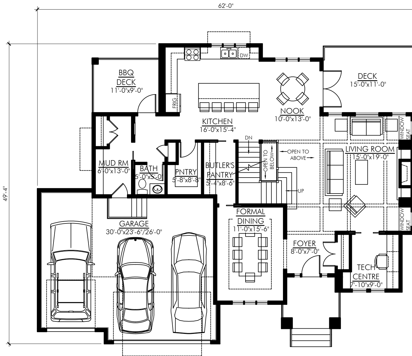
MAIN FLOOR PLAN - 1521 SQ. FT. ABBEY-3499
