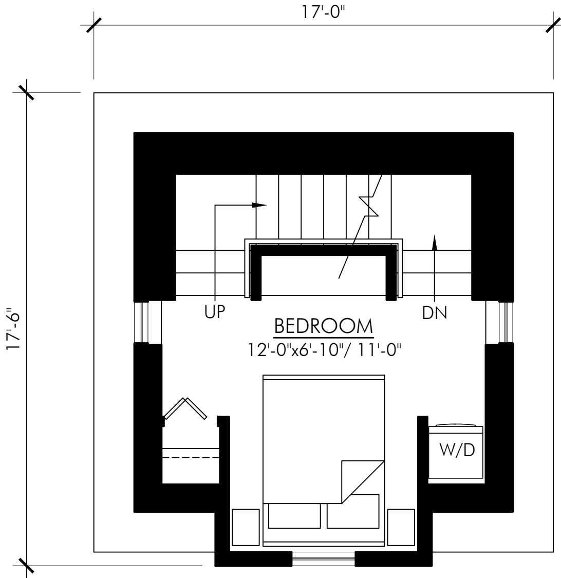
SECOND FLOOR PLAN - 169 SQ FT NOVA SCOTIA-649
