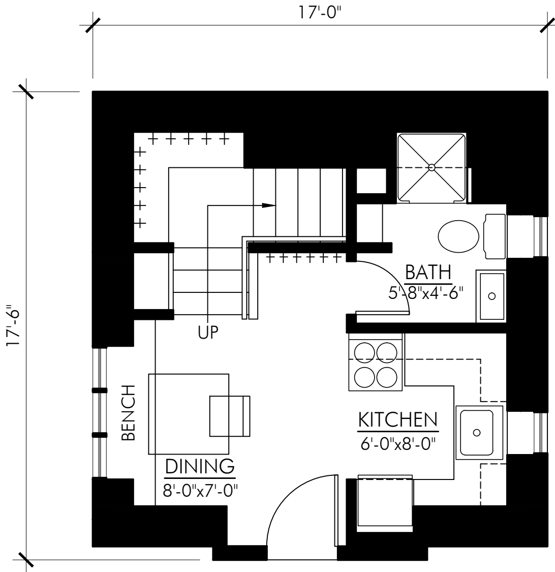
MAIN FLOOR PLAN - 293 SQ FT NOVA SCOTIA-649
