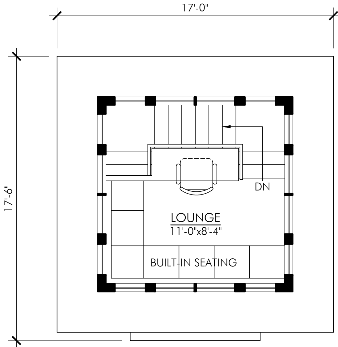
LOFT PLAN - 144 SQ FT NOVA SCOTIA-649
