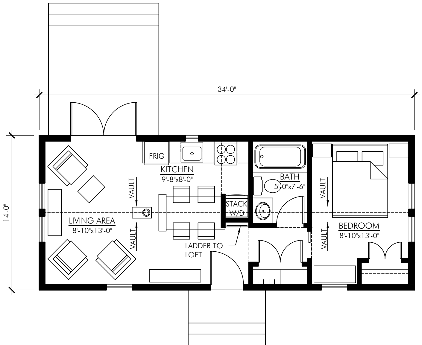
MAIN FLOOR PLAN - 476 SQ FT ONTARIO-476
