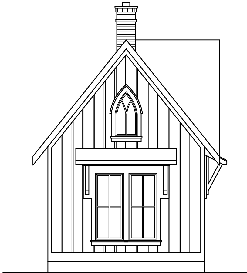
SIDE ELEVATION ONTARIO-476
