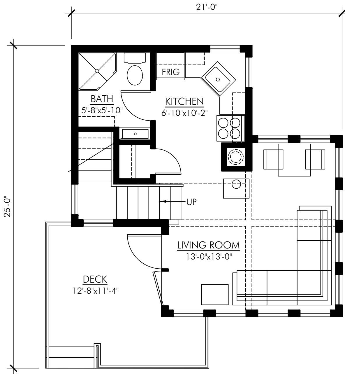
MAIN FLOOR PLAN - 343 SQ FT NORTHWEST TERRITORIES-521
