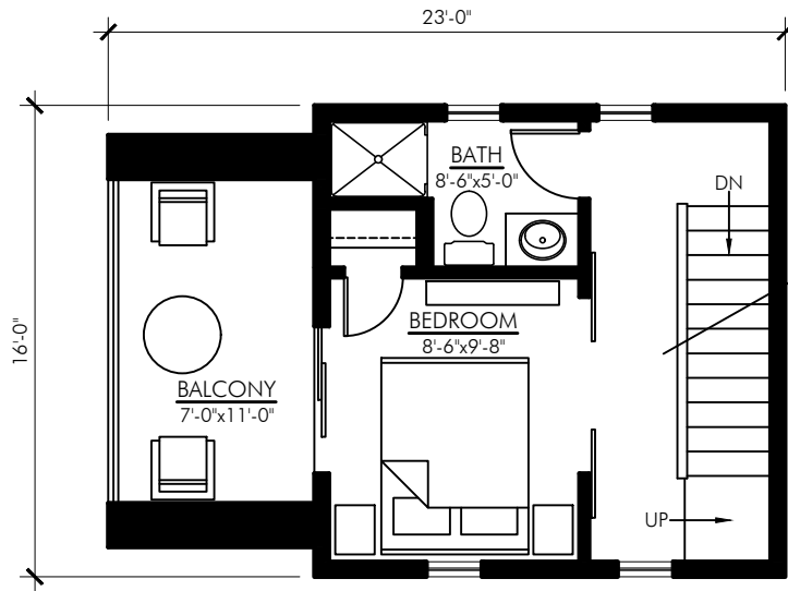
SECOND FLOOR PLAN - 256 SQ FT SASKATCHEWAN-713
