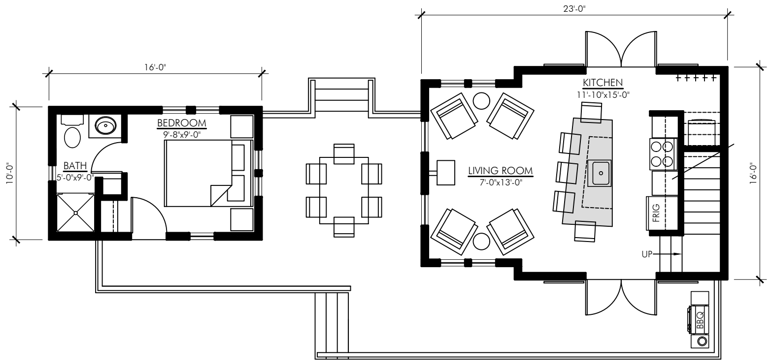
STUDIO FLOOR PLAN - 160 SQ FT SASKATCHEWAN-713
