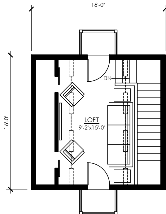
THIRD FLOOR PLAN - 103 SQ FT SASKATCHEWAN-713
