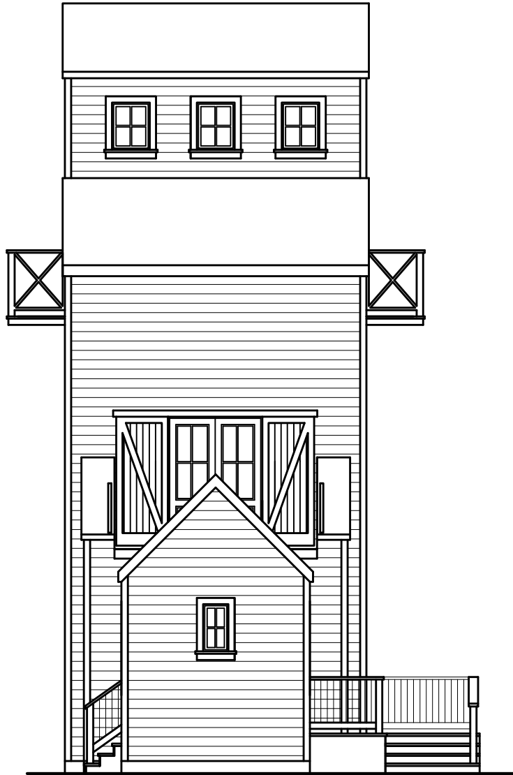
SIDE ELEVATION SASKATCHEWAN-713
